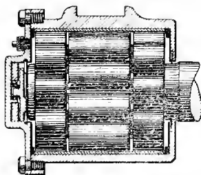
Fig. 5680. Sectional Side Elevation.
